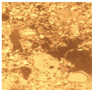
Photo1: Euhedral and Sub-euhedral coarse grains of quartz. Untreated PPL25X
